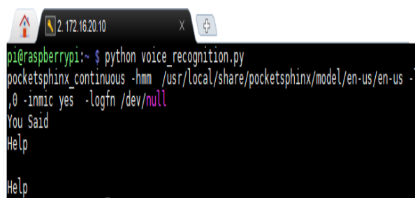
Figure 5: Voice recognition using Pocketsphinx
