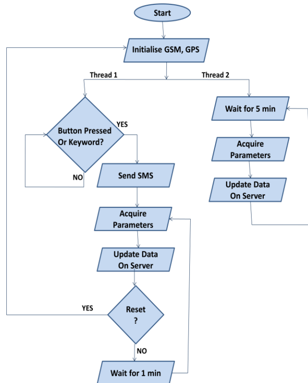
Figure 6: Design Flow
