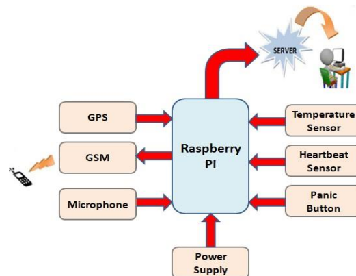
Figure 1: Block Diagram
